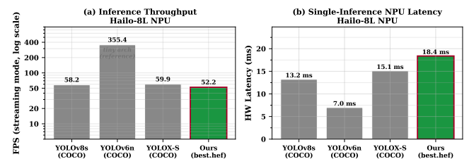
FIGURE 16. Hardware inference performance on the Hailo-8L. The custom v5 HEF runs at 52.2 FPS (18.4 ms), 6 FPS below the Hailo-provided reference (58.2 FPS, 13.2 ms); the 5 ms gap is attributable to the baked-in custom NMS, and both sit well above the 30 FPS surveillance floor.
