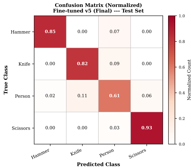
FIGURE 14. Normalised confusion matrix on the v5 held-out test set. Diagonal (recall) is 0.85, 0.82, 0.61, 0.93 for Hammer, Knife, Person, Scissors. The largest inter-class confusion is Person \rightarrow Knife at 0.11; the remainder of each true-class mass falls into the background column (missed detections), which is the dominant error mode — the safer failure mode for a security system, where a misclassified weapon still triggers an alert.
