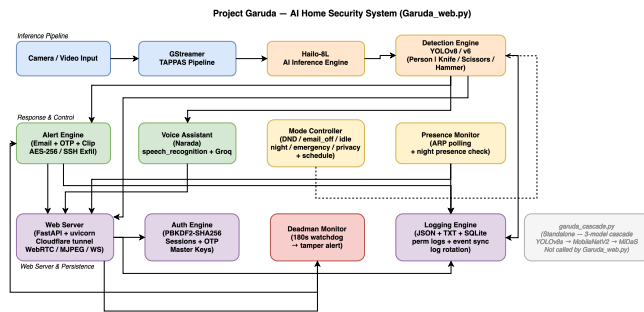
FIGURE 1. Three-layer block diagram of the proposed system. The top layer offloads all neural inference to the Hailo-8L, the middle layer routes detections through mode-gated response engines, and the bottom layer handles persistence and external access — separating concerns so that no single layer’s failure propagates upward.
