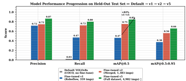
FIGURE 11. Four-model comparison on the held-out test set. COCO-pretrained YOLOv8s scores near zero on this four-class task; fine-tuning on 359 images (v1) recovers to 0.465 mAP@0.5, the intermediate v2 (1,383 images) reaches 0.754, and v5 (4,982 images) reaches 0.847 — an 82% gain over v1 driven entirely by dataset growth.
